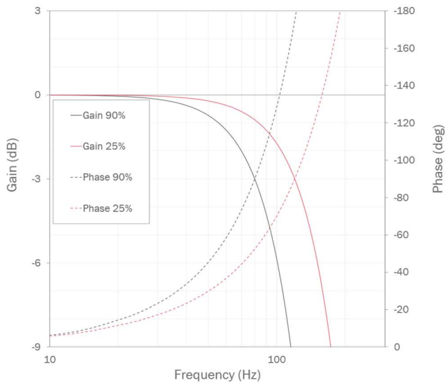
Frequency Response (1)
